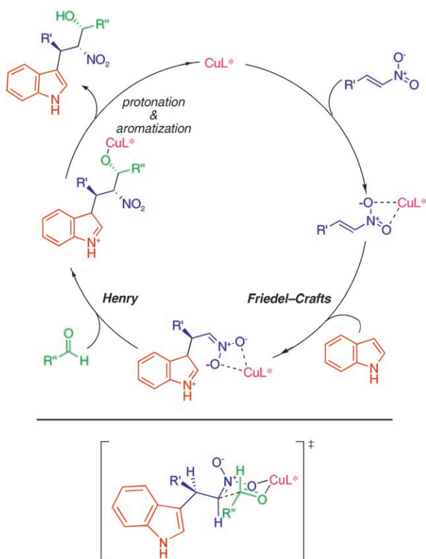
Scheme 2. Plausible reaction mechanism. \text{CuL}^* represents the 1-Cu catalyst.
